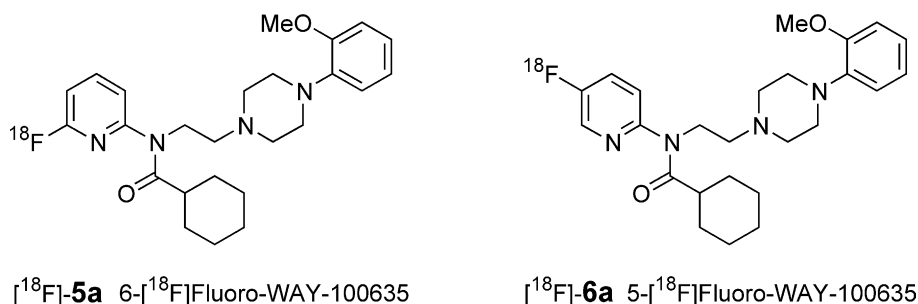
Figure 3. Chemical structures of 6-[ 18 F]fluoro- and 5-[ 18 F]fluoro-WAY-100635 ([ 18 F]- 5a/6a ).
