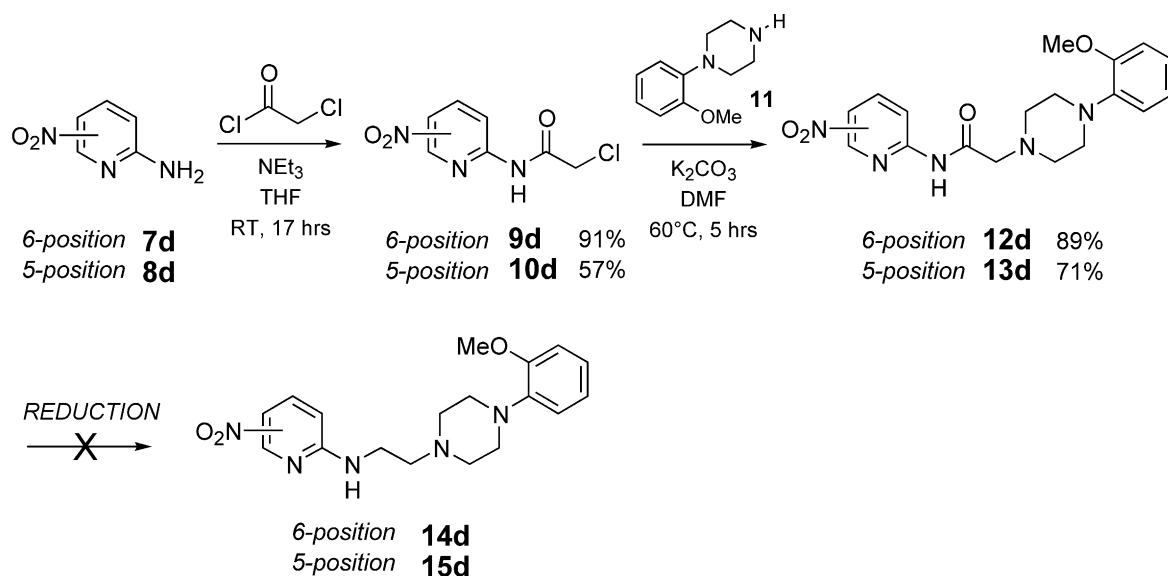
Scheme 3. Preparation of 2-[1-(4-(2-methoxyphenyl)piperazinyl)-N-(2-pyridinyl)acetamides 12d and 13d .
