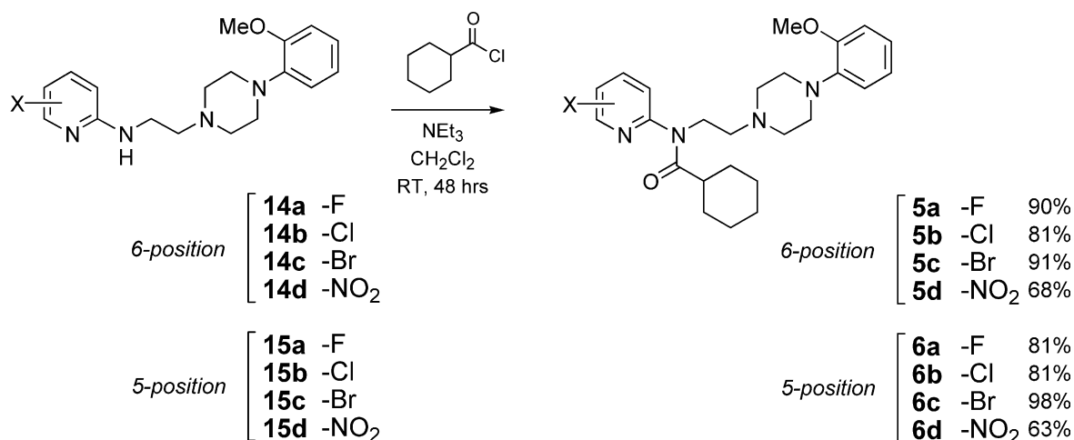
Scheme 5. Preparation of N -(2-(1-(4-(2-methoxyphenyl)piperazinyl)ethyl))- N -(2-pyridinyl)cyclohexane carboxamide 5a–d and 6a–d .
