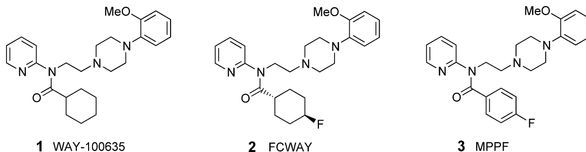
Figure 1. Chemical structures of WAY-100635 ( 1 ), FCWAY ( 2 ) and MPPF ( 3 ).
