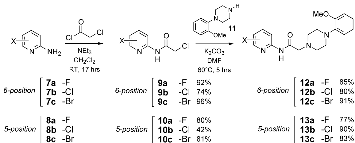
Scheme 1. Preparation of 2-[1-(4-(2-methoxyphenyl)piperazinyl)- N -(2-pyridinyl)acetamides 12a–c and 13a–c .
