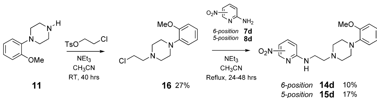
Scheme 4. Preparation of 1-(2-methoxyphenyl)-4-(2-(2-aminopyridinyl)-ethyl)piperazines 14d and 15d .
