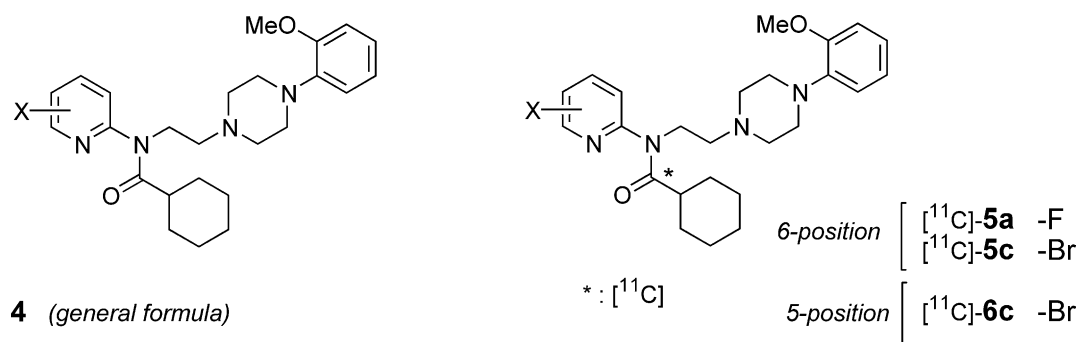
Figure 2. Chemical structures of halopyridinyl derivatives of WAY-100635 ( 4 , general formula), and in particular 6-[ 11 C]fluoro-, 6-[ 11 C]bromo- and 5-[ 11 C]bromo-WAY-100635 ([ 11 C]- 5a/5c/6c ).
