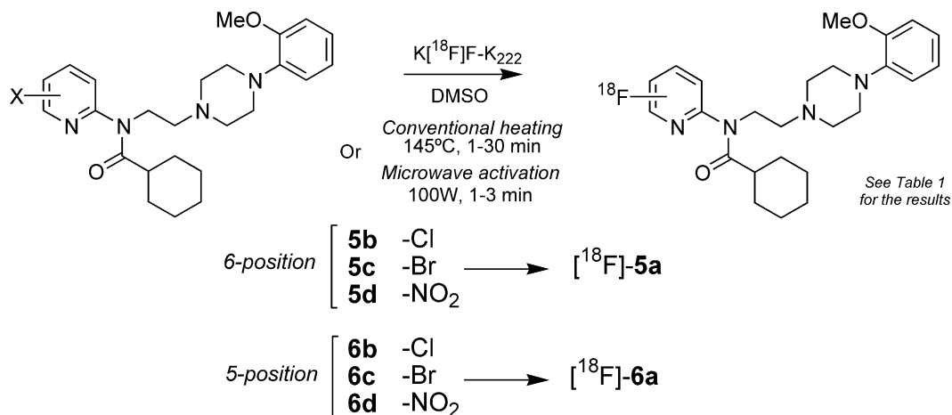
Scheme 6. Preparation of 6- ^{18}\text{F} fluoro- and 5- ^{18}\text{F} fluoro-WAY-100635 ( ^{18}\text{F} 5a / 6a ).
