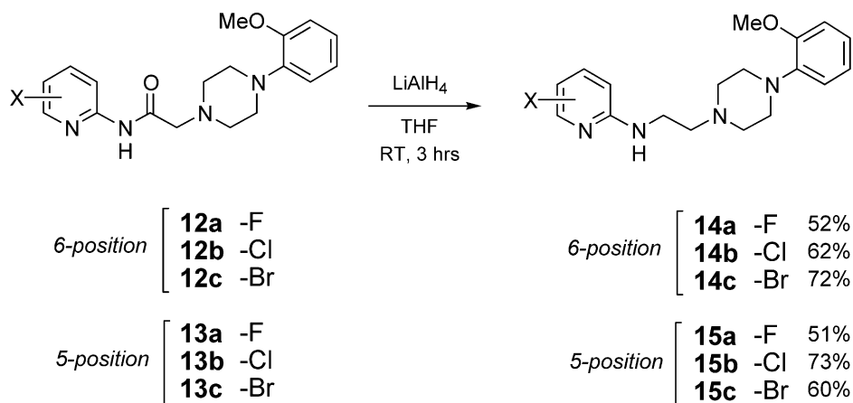
Scheme 2. Preparation of 1-(2-methoxyphenyl)-4-(2-(2-aminopyridinyl)-ethyl)piperazines 14a–c and 15a–c .
